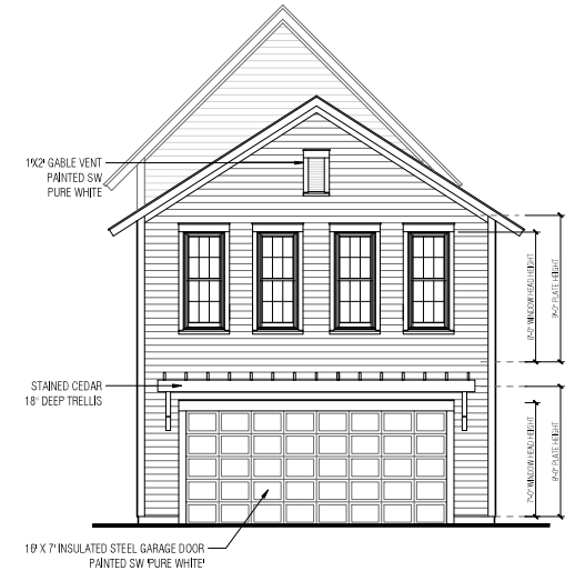
2 REAR ELEVATION SCALE 1/4" = 1'
