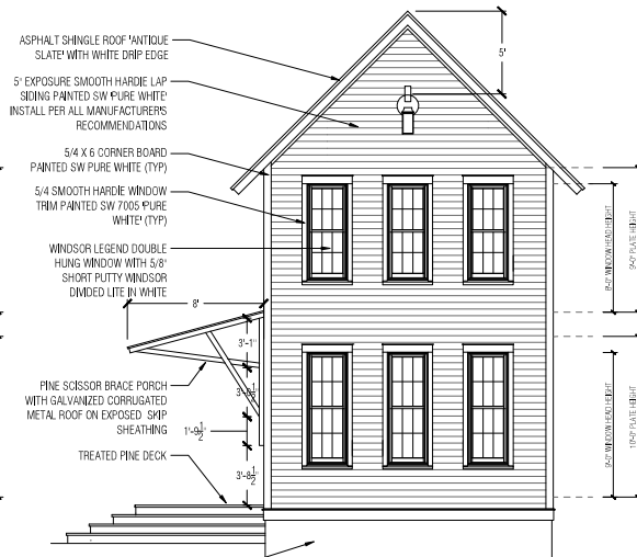
1 FRONT ELEVATION SCALE 1/4" = 1'
